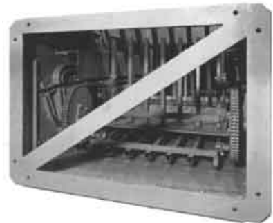
Bottom view of an 85 lb. integral trunk Vertiflo showing the mechanism which flips the return tray to its compact vertical slot return.
