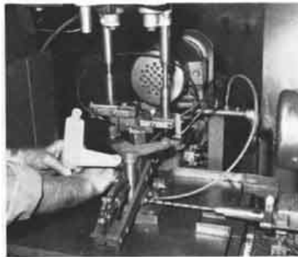
Part interchangeability assured by automatic machines.
