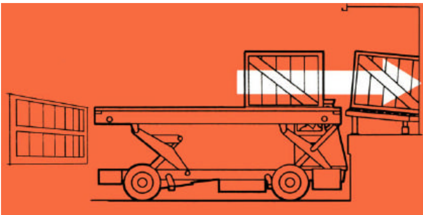
TO UNLOAD, CAB SWINGS ASIDE, CARGO DECK LIFTS TO DOCK LEVEL
